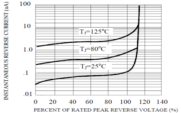
FIG. 3-TYPICAL REVERSE CHARACTERISTICS
