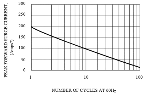
FIG. 2 - PEAK FORWARD SURGE CURRENT
