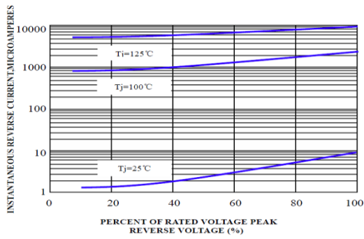
FIG. 3-TYPICAL REVERSE CHARACTERISTICS
