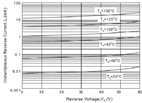
Fig. 3 - Reverse Characteristics
