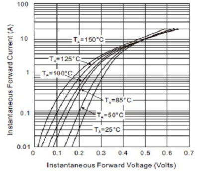
Fig. 2 - Instantaneous Forward Characteristics (per diode)
