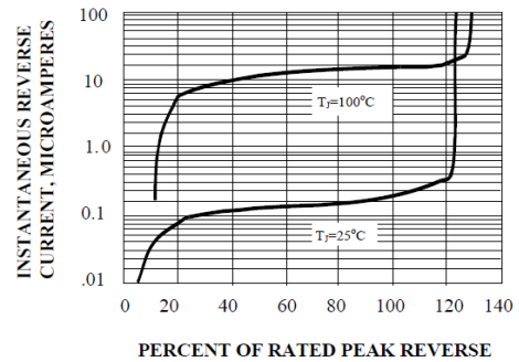
FIG. 3-TYPICAL REVERSE CHARACTERISTICS
