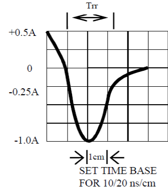
FIG. 3-TYPICAL REVERSE CHARACTERISTICS
