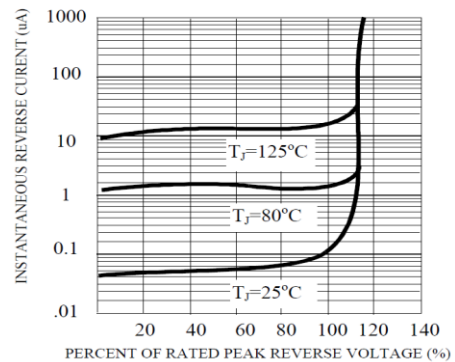
FIG. 3-TYPICAL REVERSE CHARACTERISTICS
