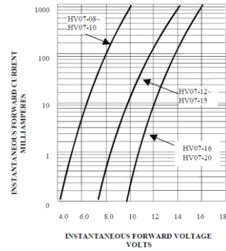
FIG. 4 - TYPICAL INSTANTANEOUS FORWARD CHARACTERISTICS
