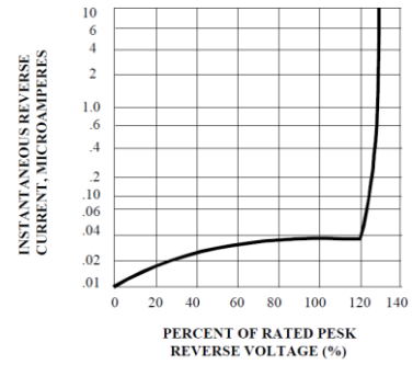
FIG. 2 - TYPICAL REVERSE CHARACTERISTICS 25°C T A
