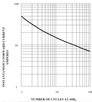
FIG. 3 - PEAK FORWARD SURGE RATING
