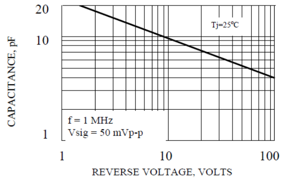
FIG. 3-TYPICAL JUNCTION CAPACITANCE
